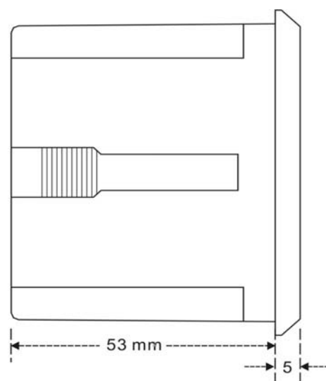
Fig. 4 GTR-17 Case Dimension of Back View
