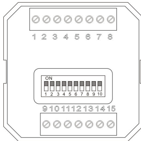
Fig. 2 GTR-117 Controller Back Panel
